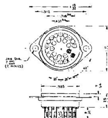
Figure 3 Contact Socket Assembly
