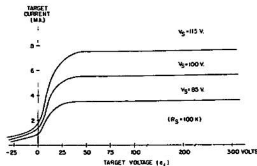
Figure 4 Output characteristic
