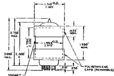
Figure 1 Outline Drawing
