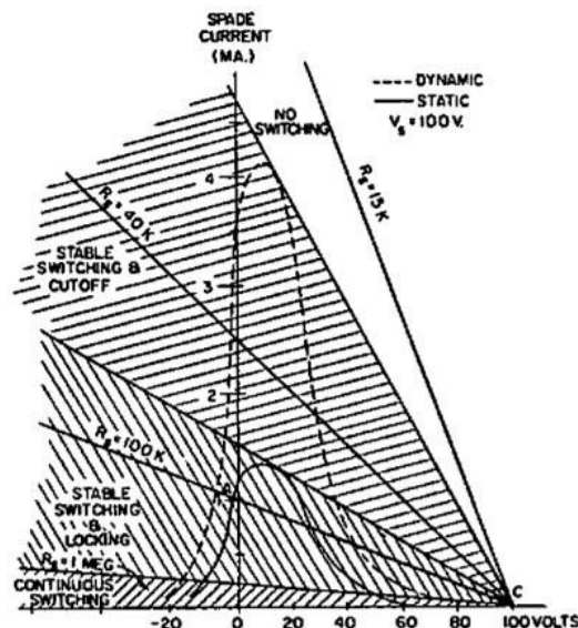
Figure 5 Beam Forming & Locking Spade Characteristic
