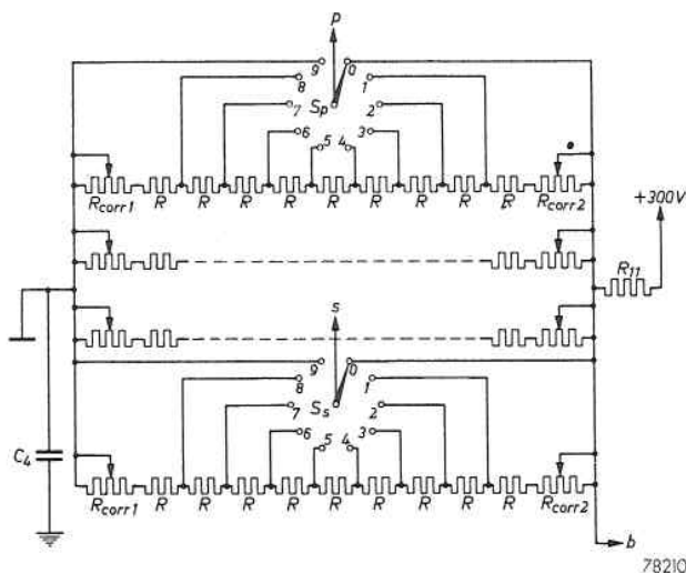
Fig. 25. Circuit for replacing the four wire-wound potentiometers P_1-P_4 and the resistors R_1-R_{10} shown in fig. 6 by fixed resistors R ( 4.7 \text{ k}\Omega \pm 2\% , \frac{1}{4} \text{ W} ) and four ten-way switches S_p-S_s . The variable resistors R_{corr} need be readjusted only when the tubes are replaced. They may be of the carbon type and should have a value of 10 \text{ k}\Omega . Only two of the four branches have been completely drawn. All resistors of this circuit should be mounted such that adequate cooling is provided, this may be done by drilling holes in the chassis above these resistors.
