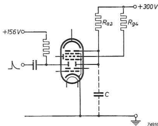
Fig. 5. Circuit for explaining the operation of the E1T counter tube, positive voltage pulses being applied to the left deflection electrode. C represents the sum of the capacitance of the anode and of the right deflection electrode with respect to all other electrodes and the wiring and stray capacitances.
