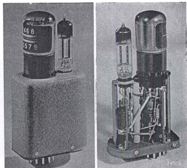
Fig. 16. Interchangeably counter unit comprising an EIT counter tube and an E90 CC double triode. The cover of the right-hand unit has been removed to show the accessory components.
