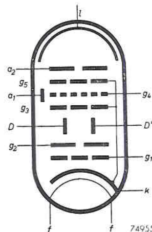
Fig. 1. (a) Cross section of the E1T counter tube. (b) Diagrammatic representation of the electrode system. For the letter references see text.
