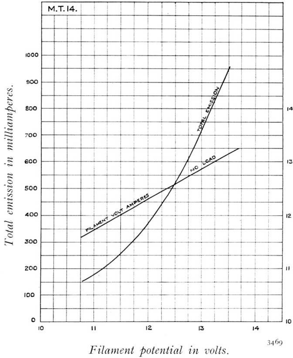
Characteristic curve of average valve.
