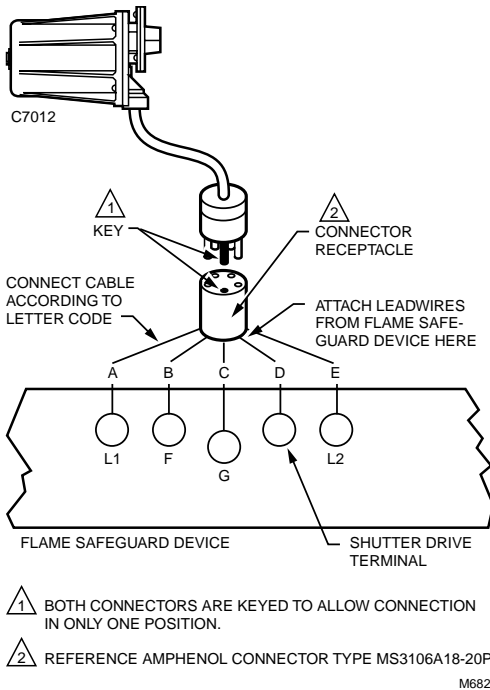
Fig. 16. Wiring connection for C7012E1161 or C7012E1278.
