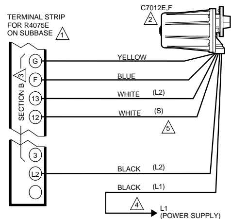
Fig. 10. Wiring diagram for C7012E or F Detectors with R4075C or D (currently obsolete) Flame Safeguard Controls.
