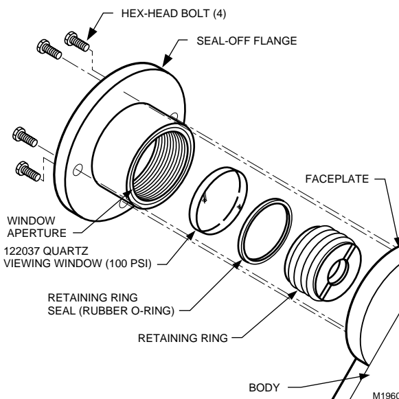
Fig. 23. Replacing quartz viewing window on C7012C,F.
