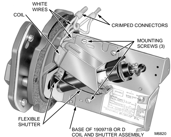
Fig. 21. Replacing coil and shutter assembly on C7012E,F.
