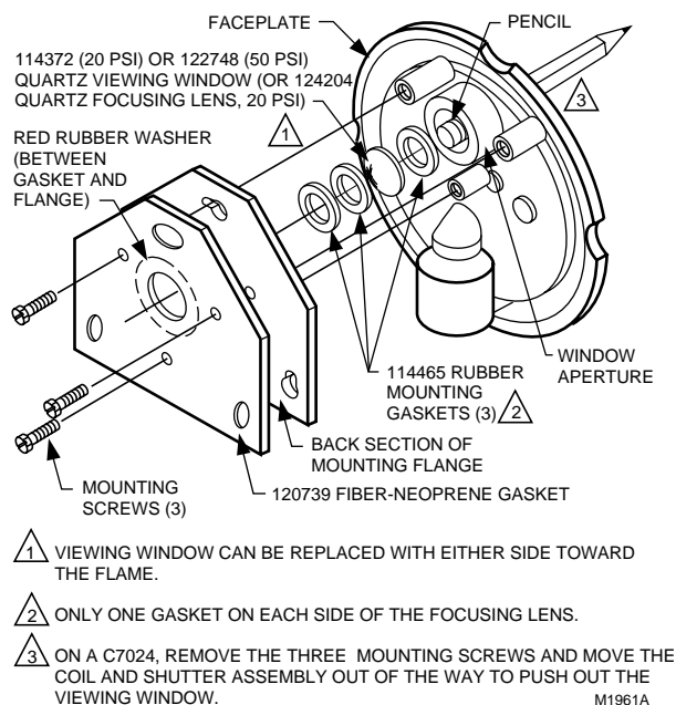
Fig. 22. Replacing quartz viewing window or focusing lens on C7012A,E,G.
