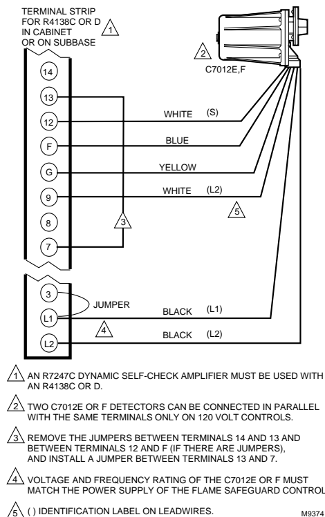
Fig. 12. Wiring diagram for C7012E or F Detectors with R4138C,D (currently obsolete) Flame Safeguard controls.
