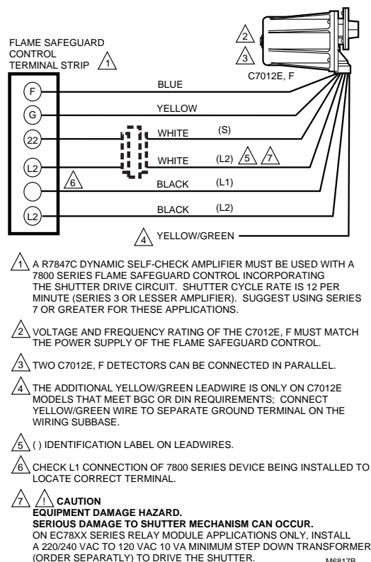
Fig. 15. Wiring diagram for C7012E,F Detectors with 7800 SERIES Flame Safeguard Controls with shutter drive circuitry.
