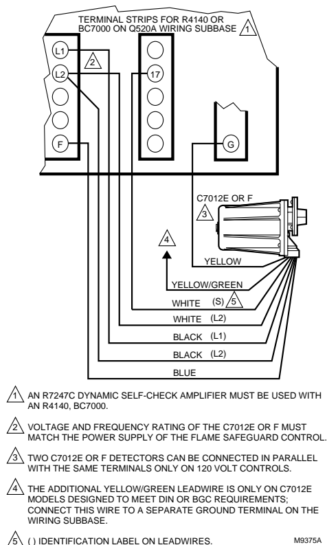
Fig. 13. Wiring diagram for C7012E or F Detectors with R4140 and BC7000 Flame Safeguard controls.
