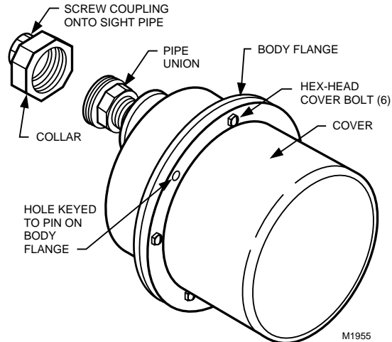
Fig. 8. Mounting C7012C or F Detector.
