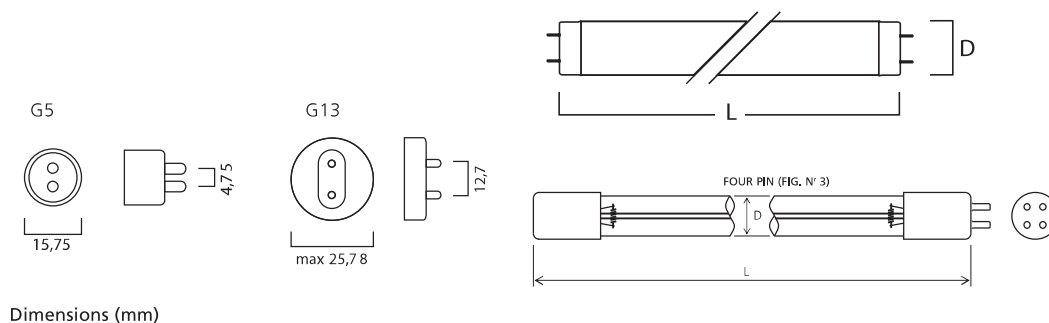
Dimensions (mm)
