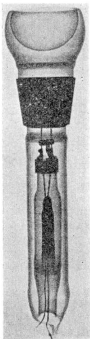
Fig. 3. Grenz-ray tube with Slack window.
