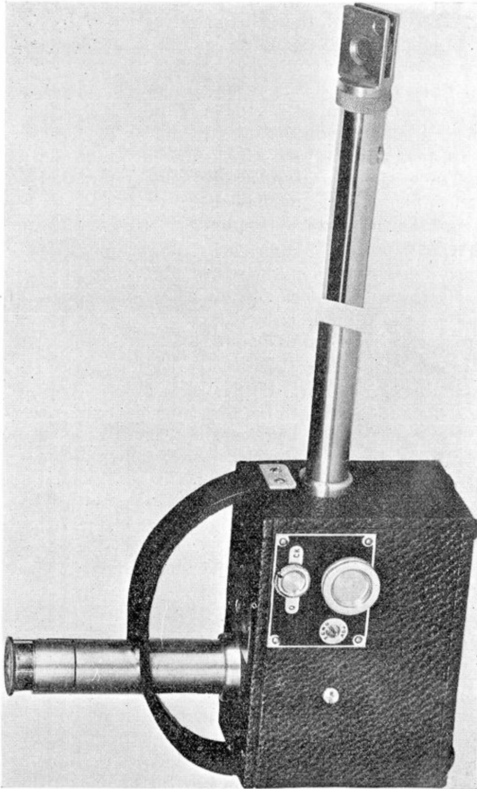
Fig. 10. Victoreen r meter with Grenz-ray chamber.
