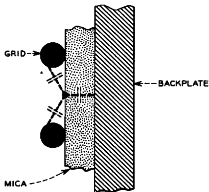
Fig. 3 — Capacitance distribution between the barrier grid, the dielectric surface, and the backplate.
