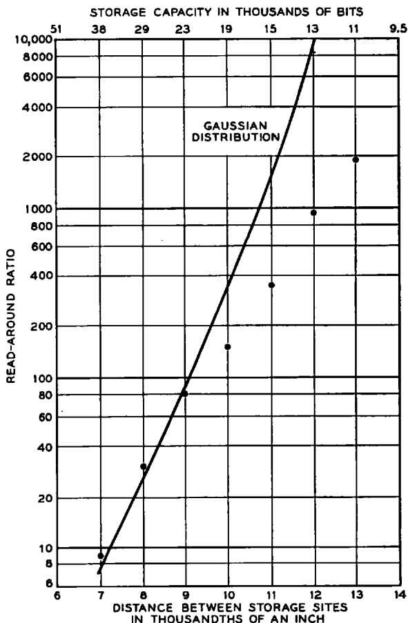
Fig. 11 — Read-around ratio and storage capacity as a function of the distance between adjacent storage sites.
