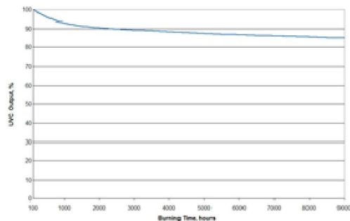
Maintenance Curve
